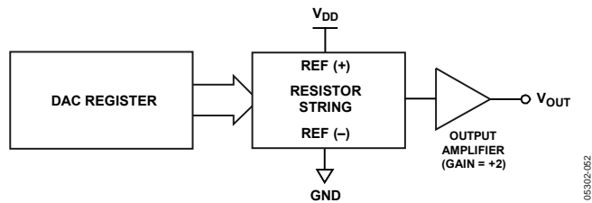
Figure 51. DAC Architecture
