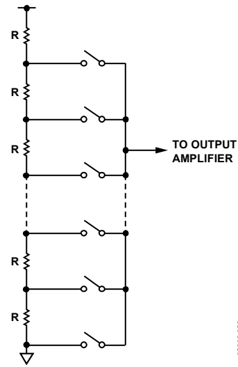
Figure 52. Resistor String
